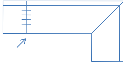
Butt Joint
